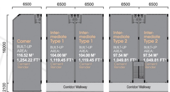
F First Floor Plan
