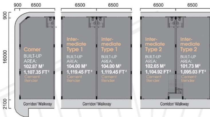
G Ground Floor Plan
